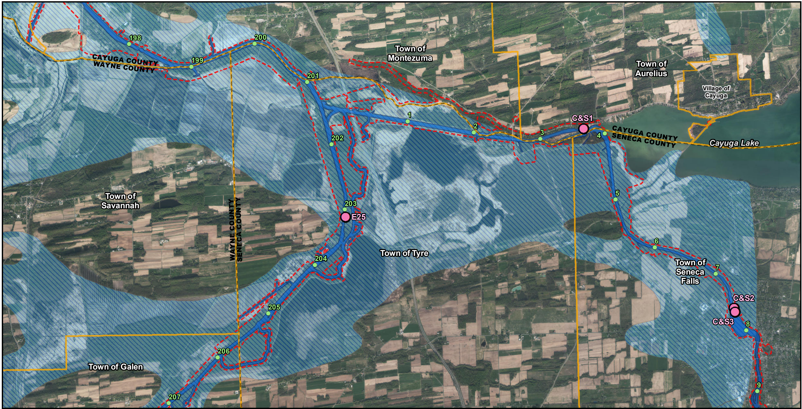
Figure 86F: Aquifers
